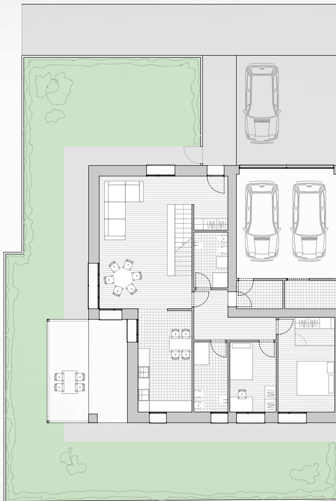
Piano terra
